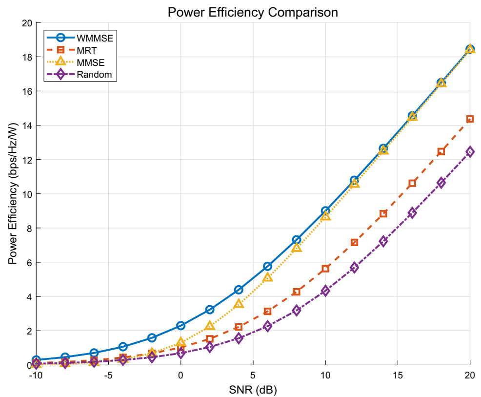
Fig. 5 System energy efficiency versus SNR
