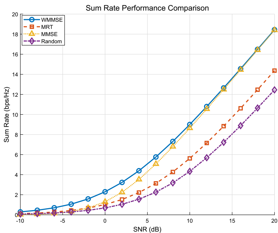
Fig. 2 System sum-rate versus SNR
