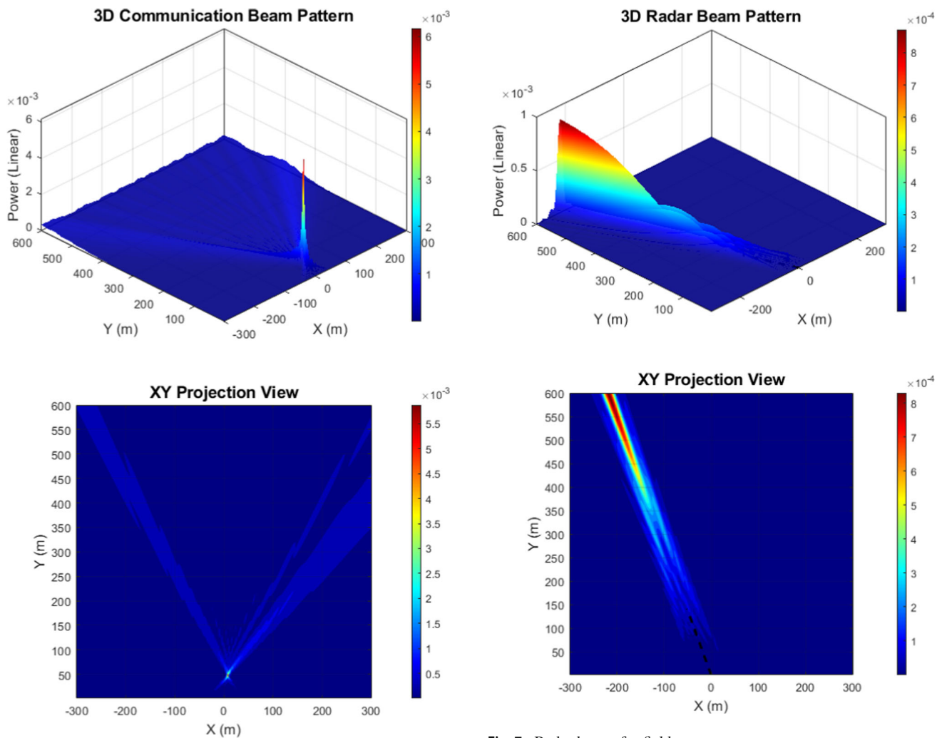
Fig. 7 Radar beam: far-field
